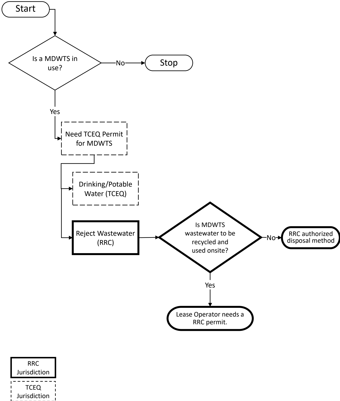
Figure 2: Mobile Drinking Water Treatment System (MDWTS) Permitting / Jurisdiction
